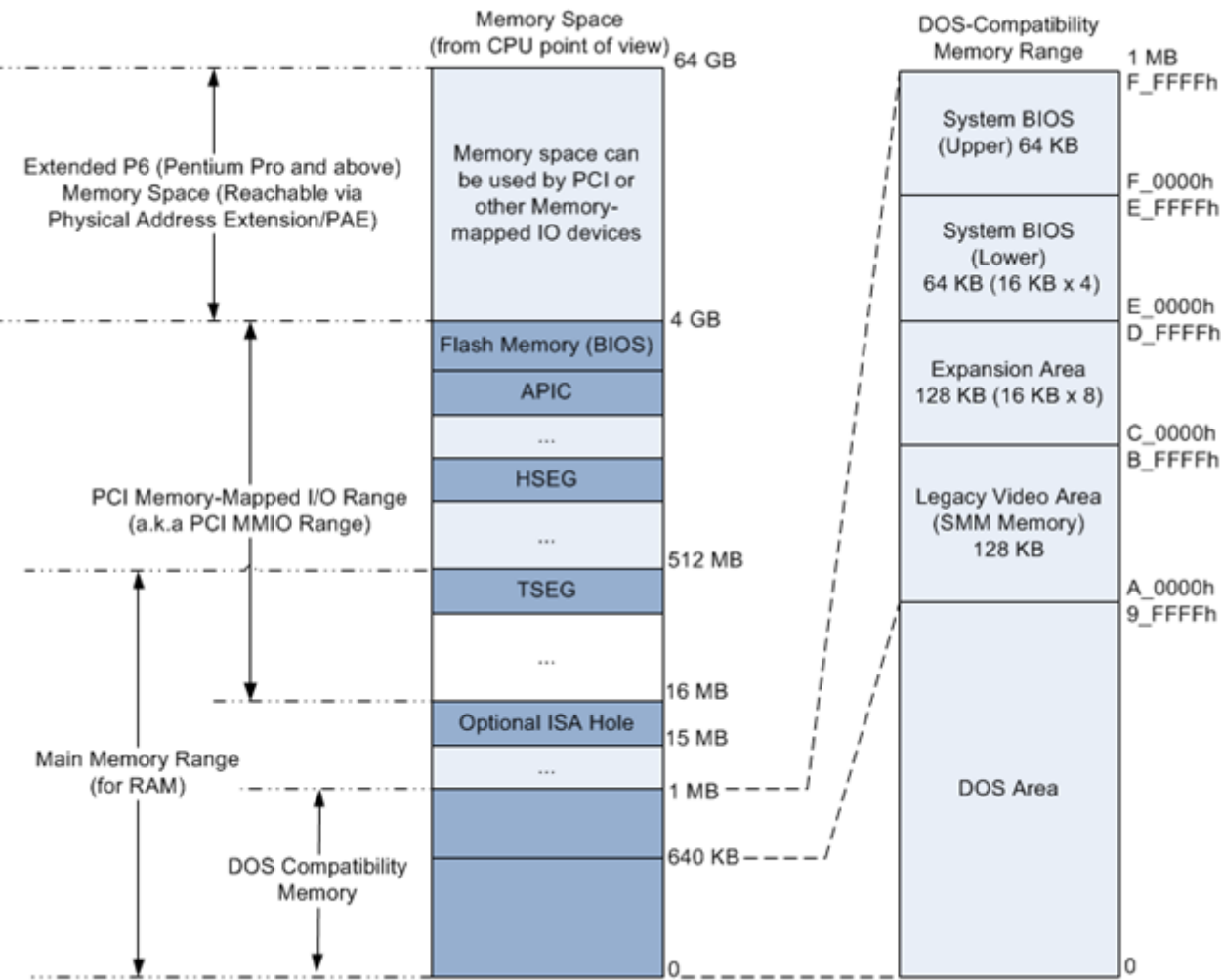
Figure 2 Intel 815E System Address Map
