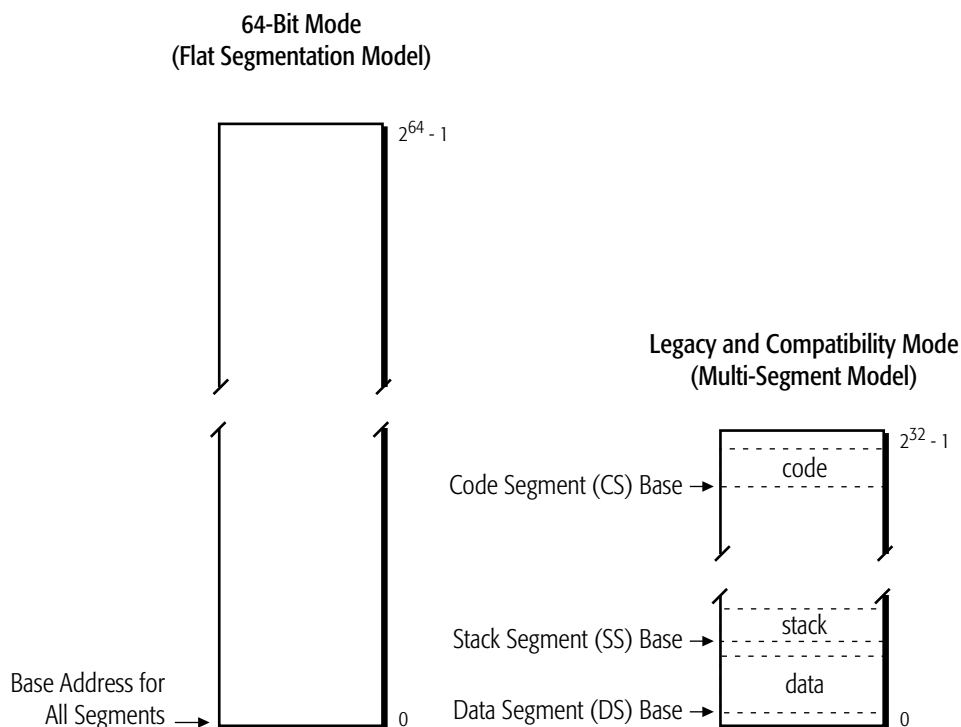
Figure 2-1. Virtual-Memory Segmentation
