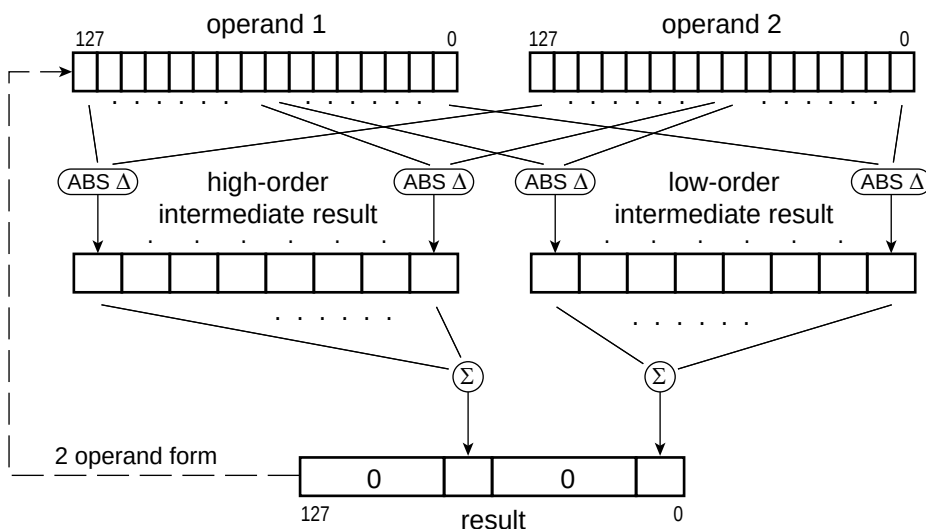
Figure 4-20. Sum-of-Absolute-Differences Operation
