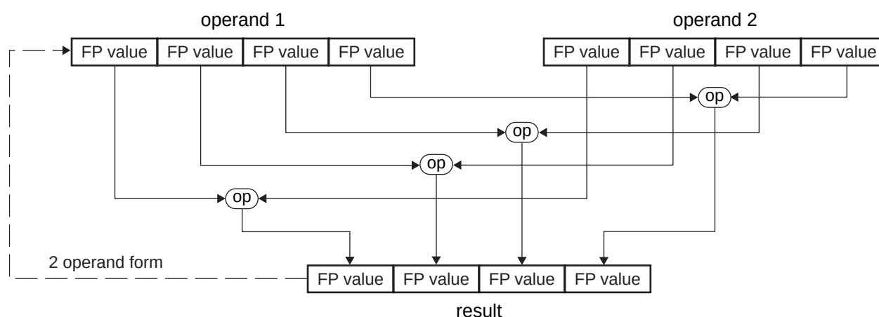
Figure 4-44. Vector Arithmetic Operation
