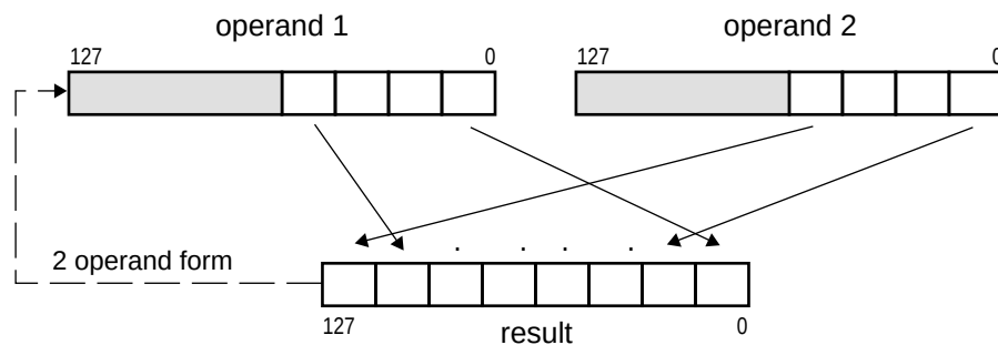
Figure 4-27. (V)PUNPCKLWD Unpack and Interleave Operation
