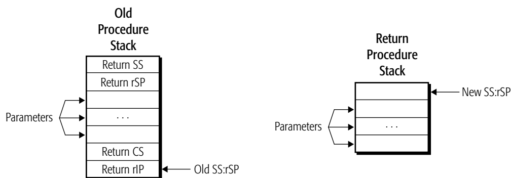
Figure 3-15. Procedure Stack, Far Return from Less Privilege
