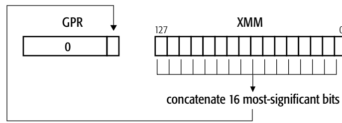
Figure 4-25. (V)PMOVMASKB Move Mask Operation
