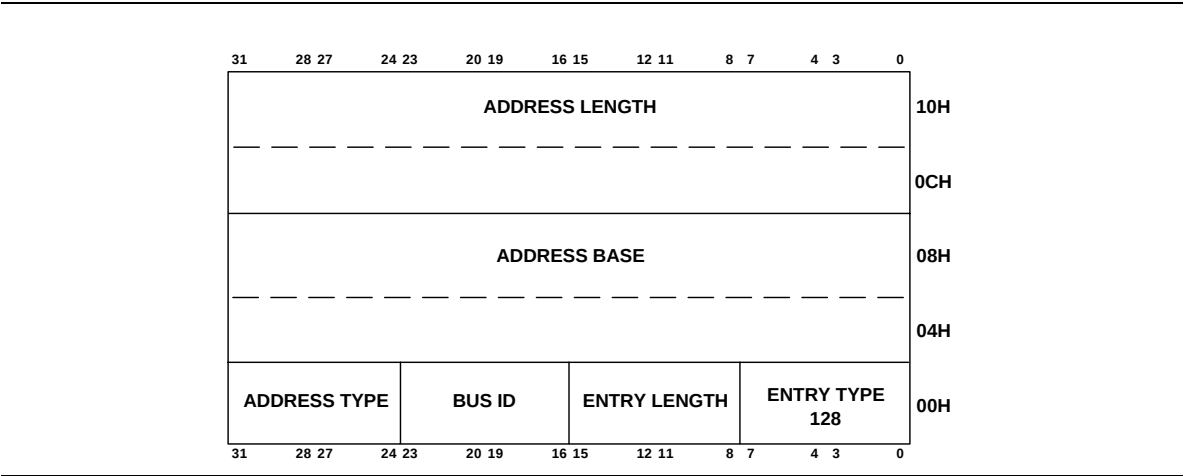
Figure 4-9. System Address Space Entry
