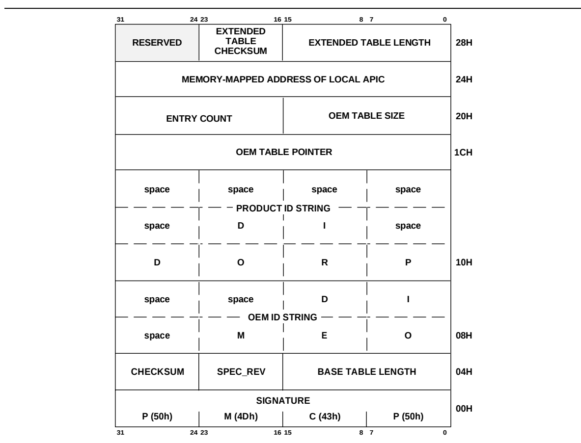
Figure 4-3. MP Configuration Table Header
